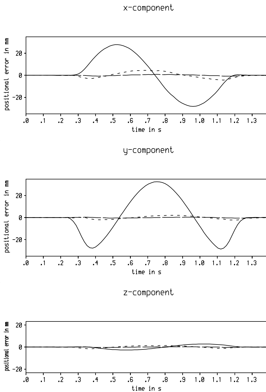
Figure 5. Pose error of a horizontal circular path before learning (solid), after the first iteration (dotted), and after the second iteration (dashed)
