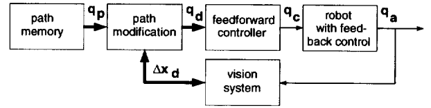
Figure 2: Indirect control architecture
