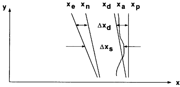
Figure 3: Notation of different paths ( x_p = original desired path, x_d = sensed desired path, x_a = actual path, x_e = actual edge, x_n = nominal edge, \Delta x_s = sensor value, \Delta x_d = modification of the desired path due to a difference between the nominal and the actual edge)
