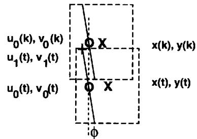
Figure 5: Calculation of the sensor orientation \phi(k) from two images at time instants k and t ( x = \text{TCP} , o = \text{edge at TCP} , + = \text{edge at future position} )
