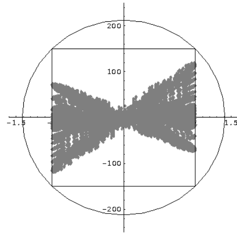
Fig. 11. Projection to force dimensions 2 and torque dimension 4. The box is the projection of the Hull(\overline{OWS}) , the outer circle is the projection of the enclosing ellipsoid, resulting from Q . (Note that the plot axes are scaled so that the outer ellipsoid is mapped to a circle)
