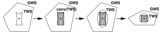
Fig. 7. Approximating the OWS with an ellipsoid:
