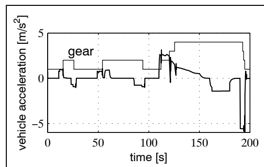
Figure 16: Vehicle acceleration and actual gear.
